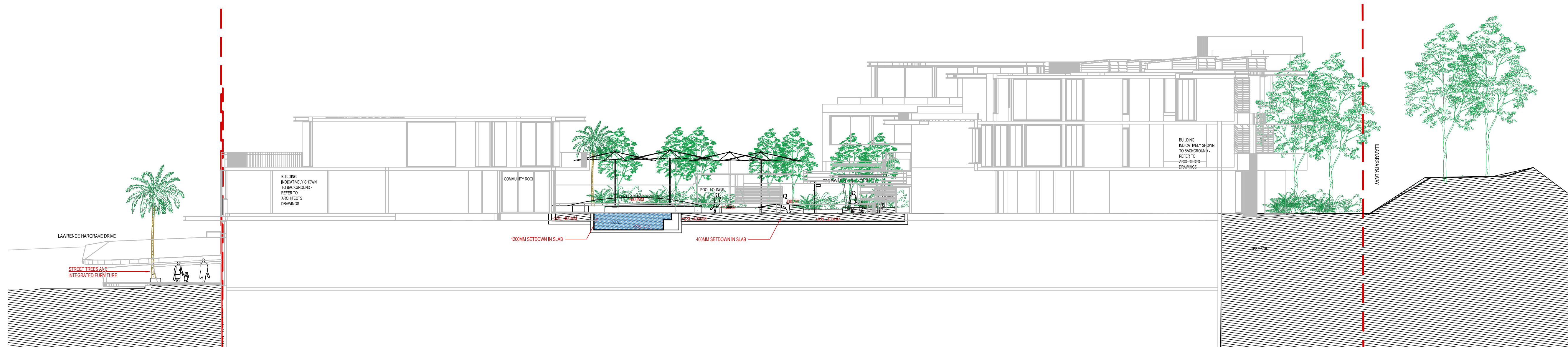
SECTION BB: 1-100 @A1
